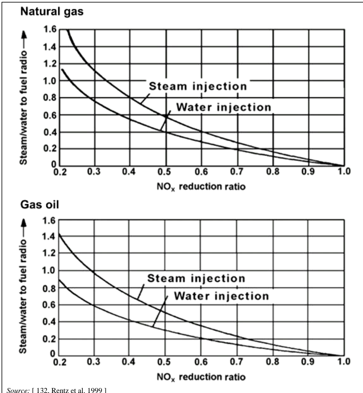
Figure 3.40: \text{NO}_x reduction by steam or water injection
