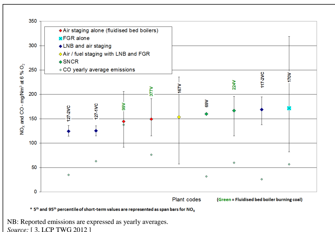
Figure 5.38: \text{NO}_x emissions from well-performing pulverised lignite boilers and coal or lignite fluidised bed boilers of more than 300 \text{ MW}_{\text{th}}
