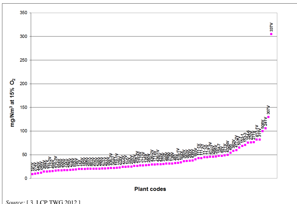
Figure 7.15: NO x emissions (yearly averages) from CCGTs without supplementary firing at the HRS level
