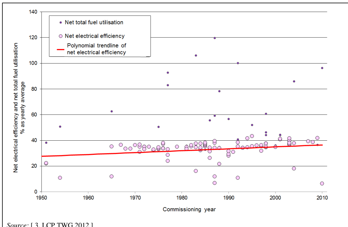
Figure 5.15: Efficiency of coal- and/or lignite-fired power plants in Europe in relation to the commissioning year based on operating yearly average energy efficiency values
