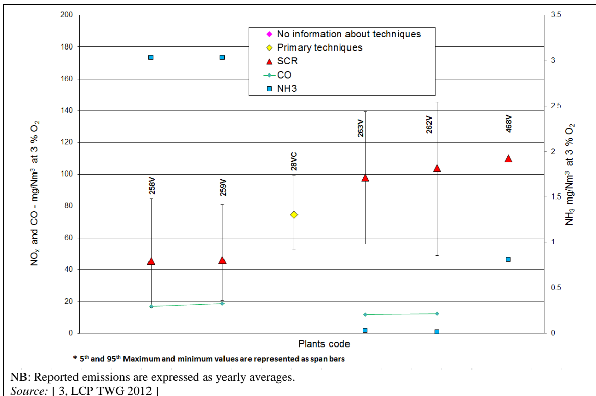
Figure 6.3: \text{NO}_x emissions from well-performing HFO- and/or gas-oil-fired boilers of \geq 100 \text{ MW}_{\text{th}}
