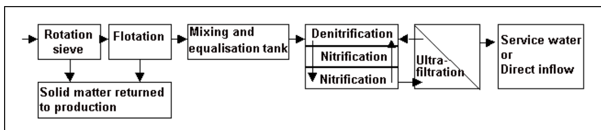
Figure 4.16: Flow diagram of biological waste water treatment using overpressure in conjunction with ultrafiltration
