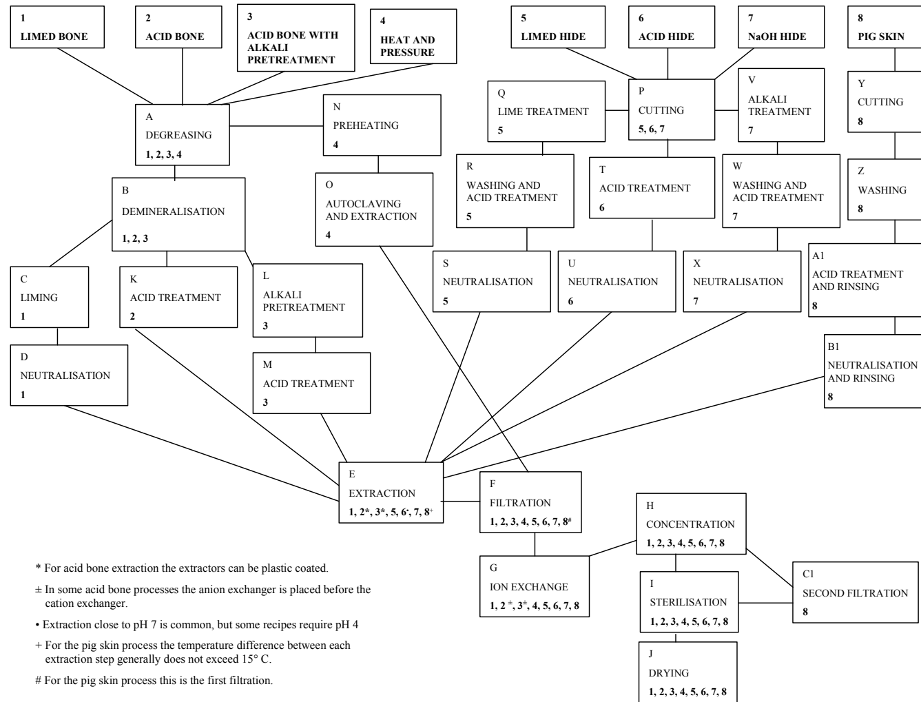
Figure 2.11: The main gelatine manufacturing processes [249, GME, 2002]
