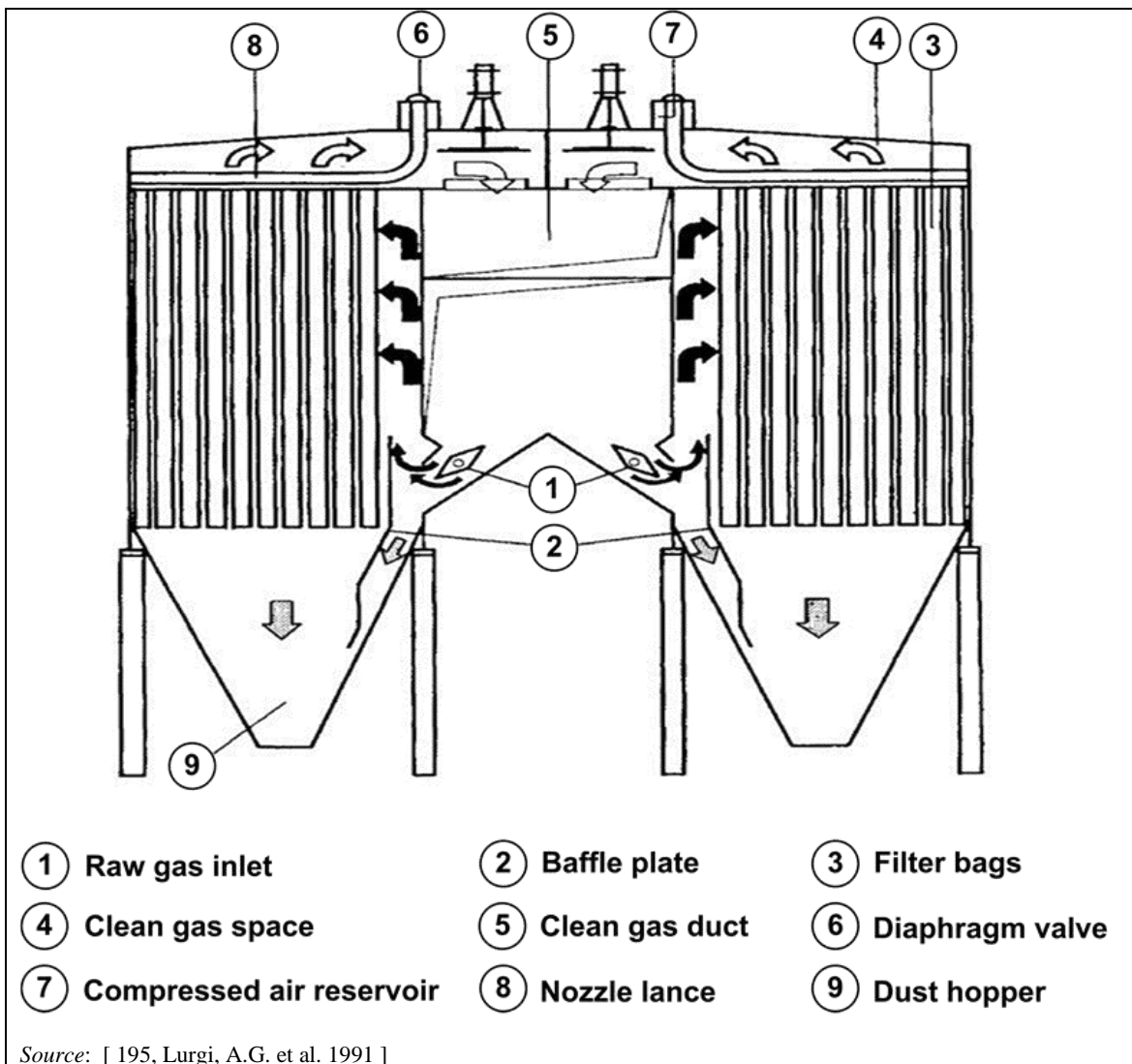
Figure 2.27: Reverse pulse jet cleaning system
