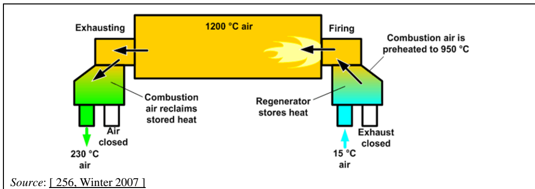
Figure 2.15: Second half of the regenerative burner cycle
