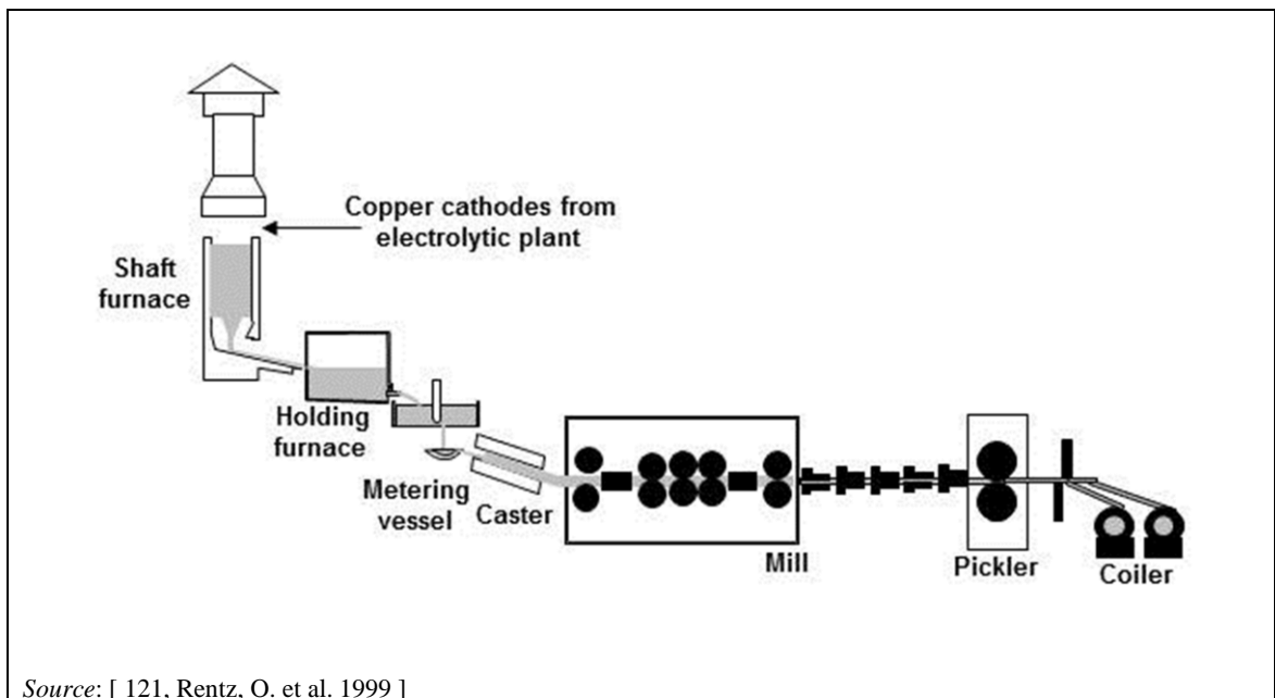
Figure 3.5: Example of the Contirod process
