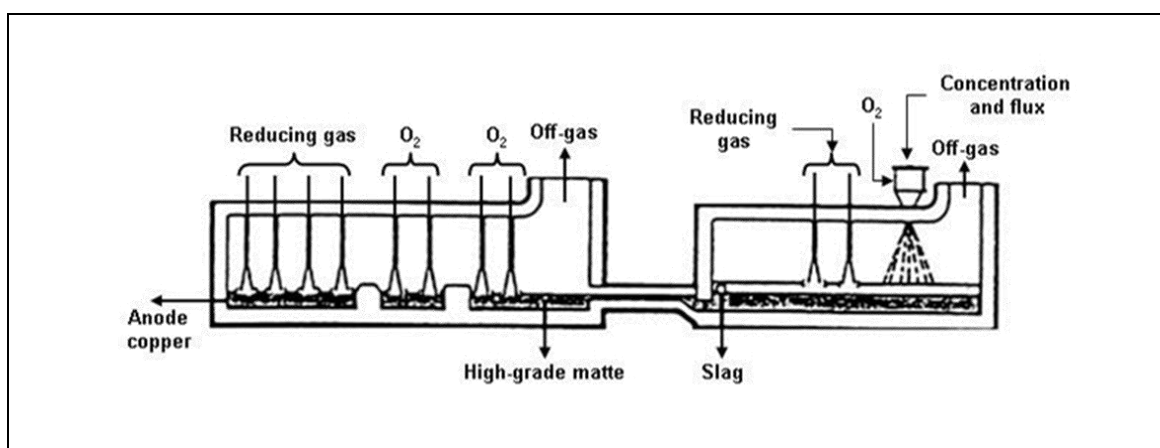
Figure 13.18: The Contop process
