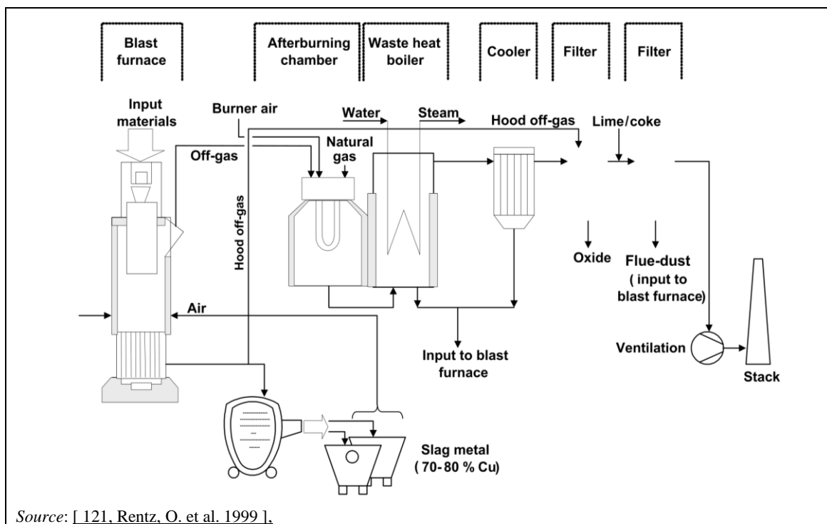
Figure 13.7: Blast furnace for secondary copper production
