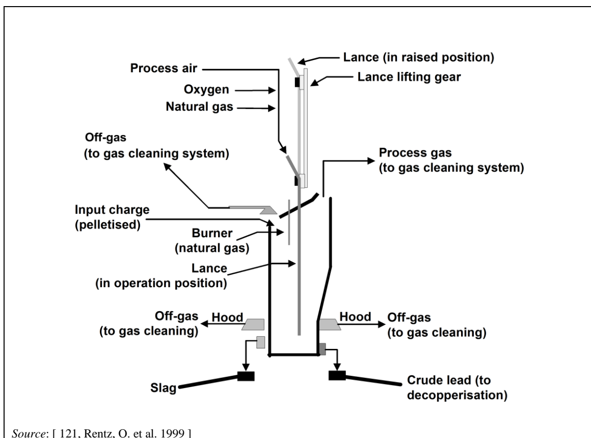
Figure 13.12: The Ausmelt (Sirosmelt)/ISASMELT furnace
