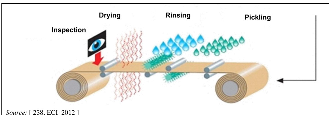
Figure 3.16: Continuous pickling process
