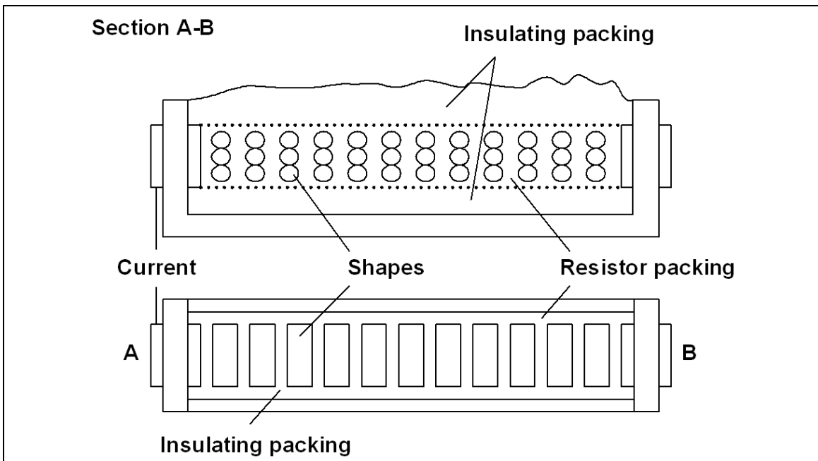
Figure 10.5: Acheson graphitising furnace
