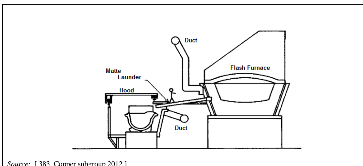
Figure 3.14: Local hood for matte tapping at the Toyo smelter
