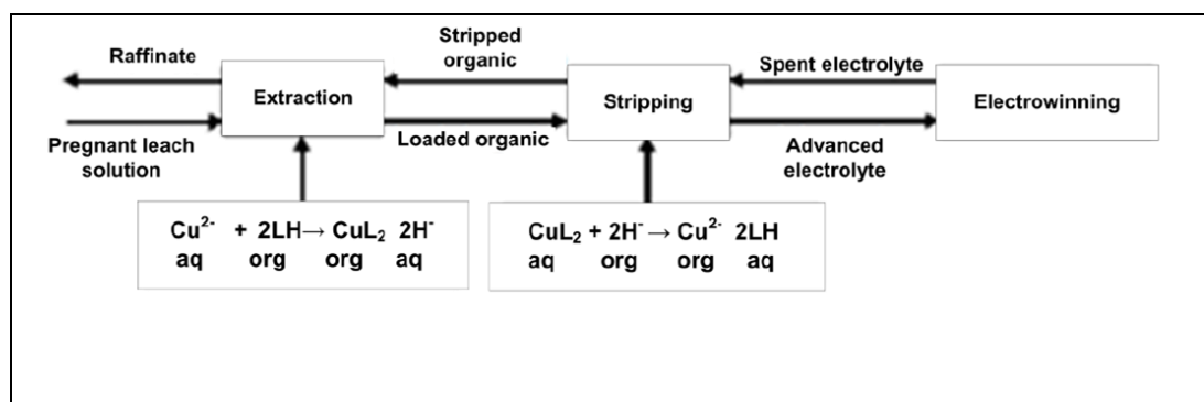
Figure 13.26: Solvent extraction (SX) processing stages
