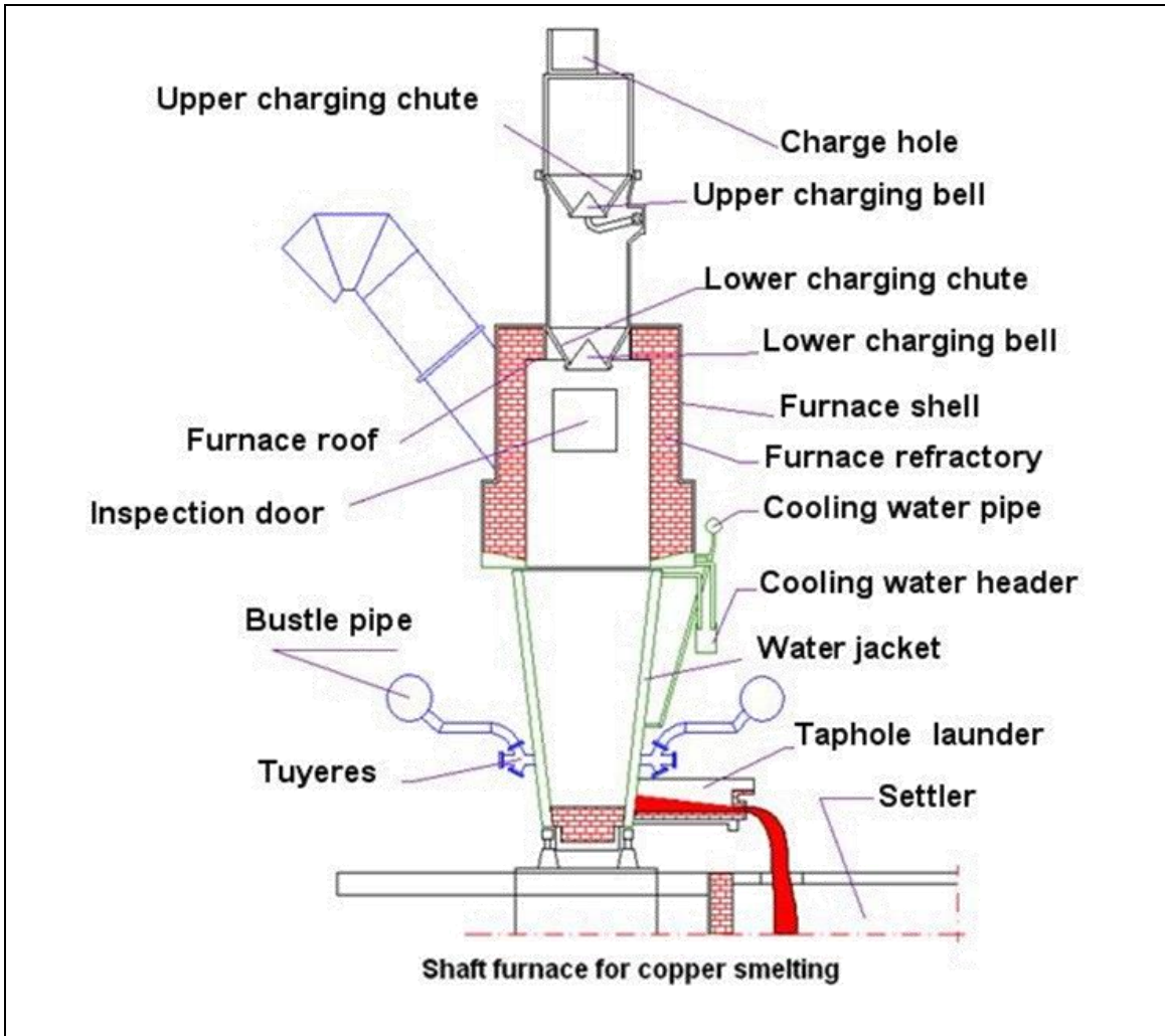
Figure 13.6: Blast furnace for primary copper smelting
