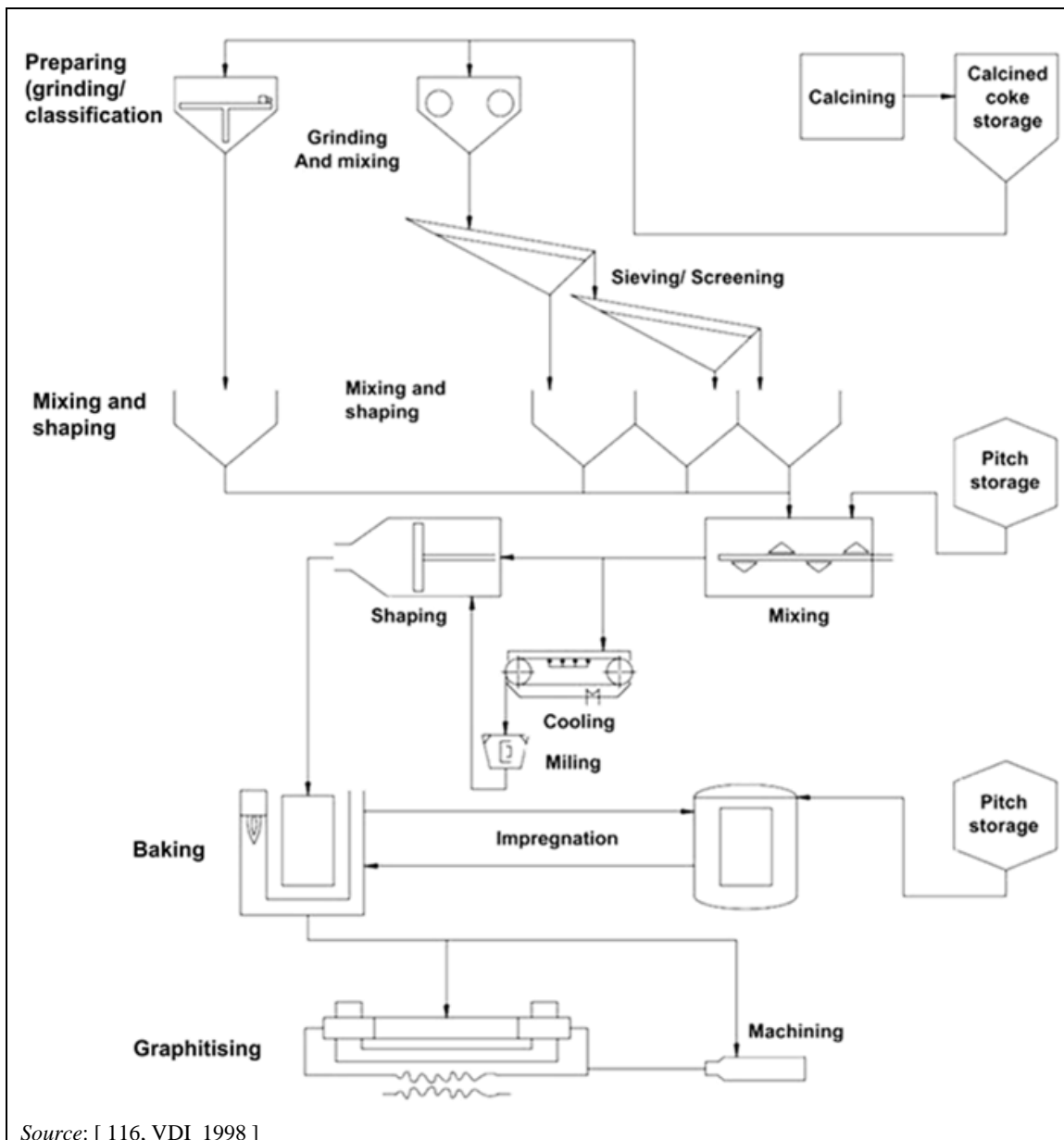
Figure 10.1: Overview of carbon and graphite production
