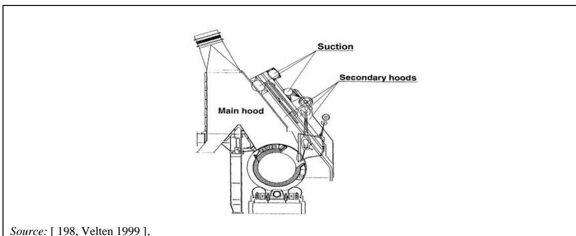
Figure 3.15: Secondary hooding system for a converter
