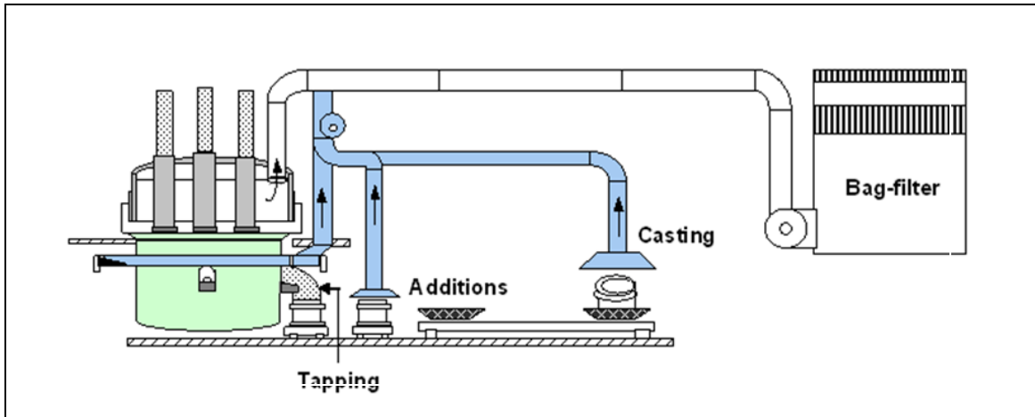
Figure 2.18: Fourth hole fume collection
