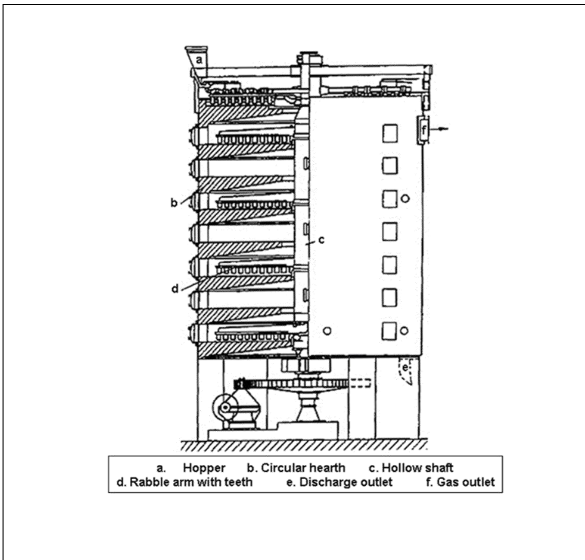
Figure 13.3: The Herreshoff or multiple hearth furnace
