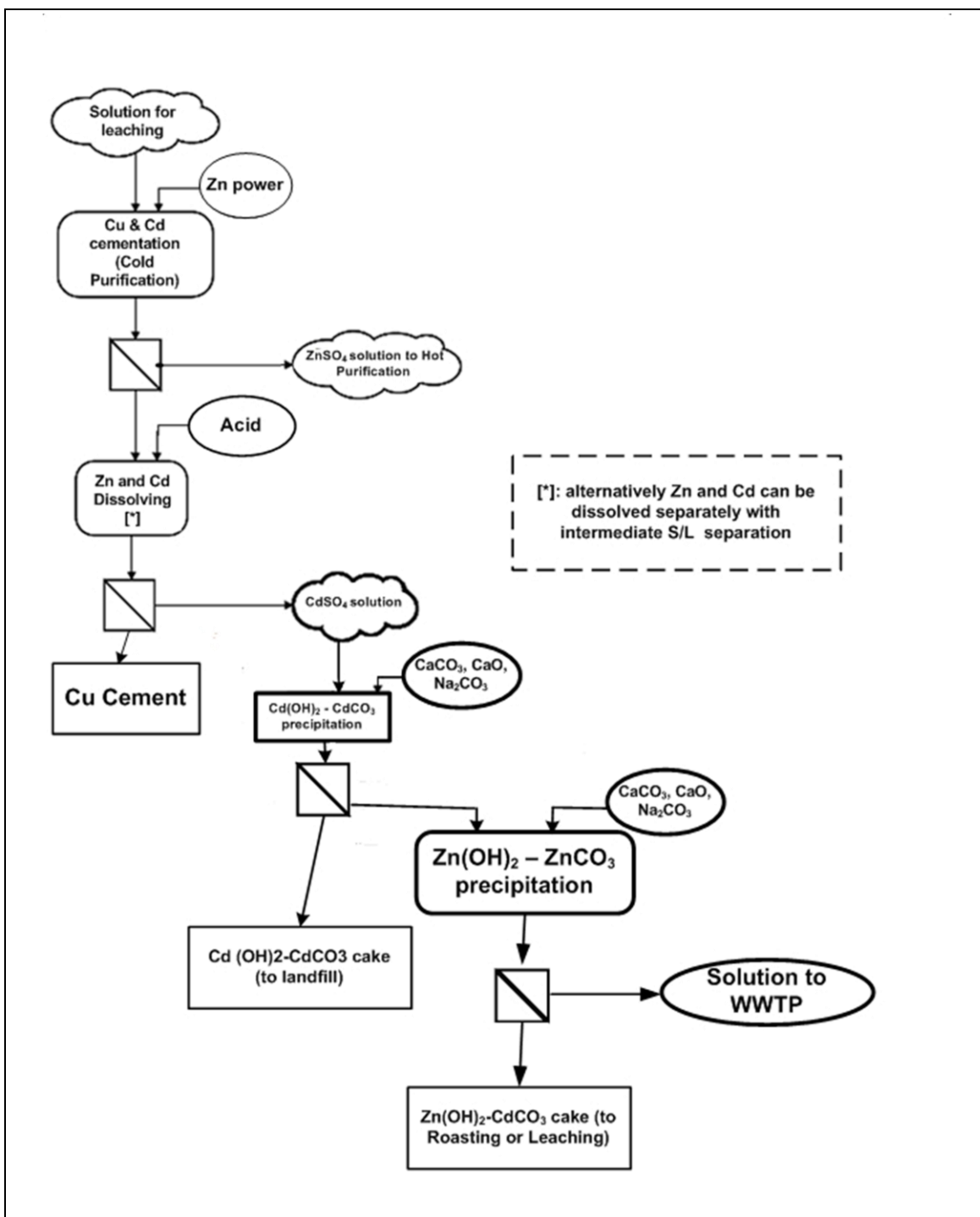
Figure 6.19: Cadmium production flowsheet: Plant E
