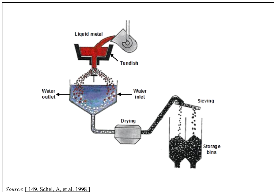
Figure 2.9: Granulation of molten metal
