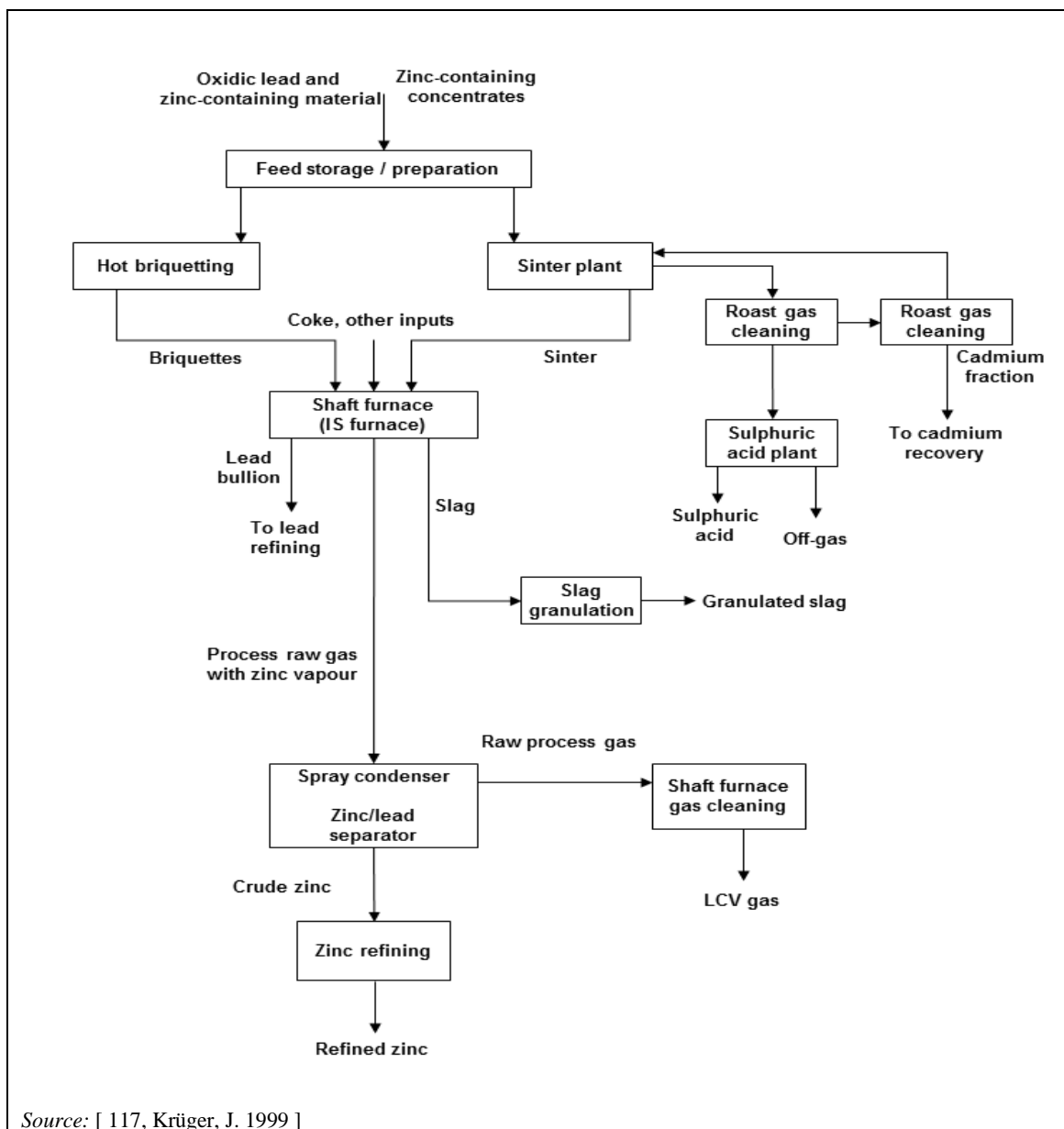
Figure 6.1: Diagram of a typical Imperial Smelting Process
