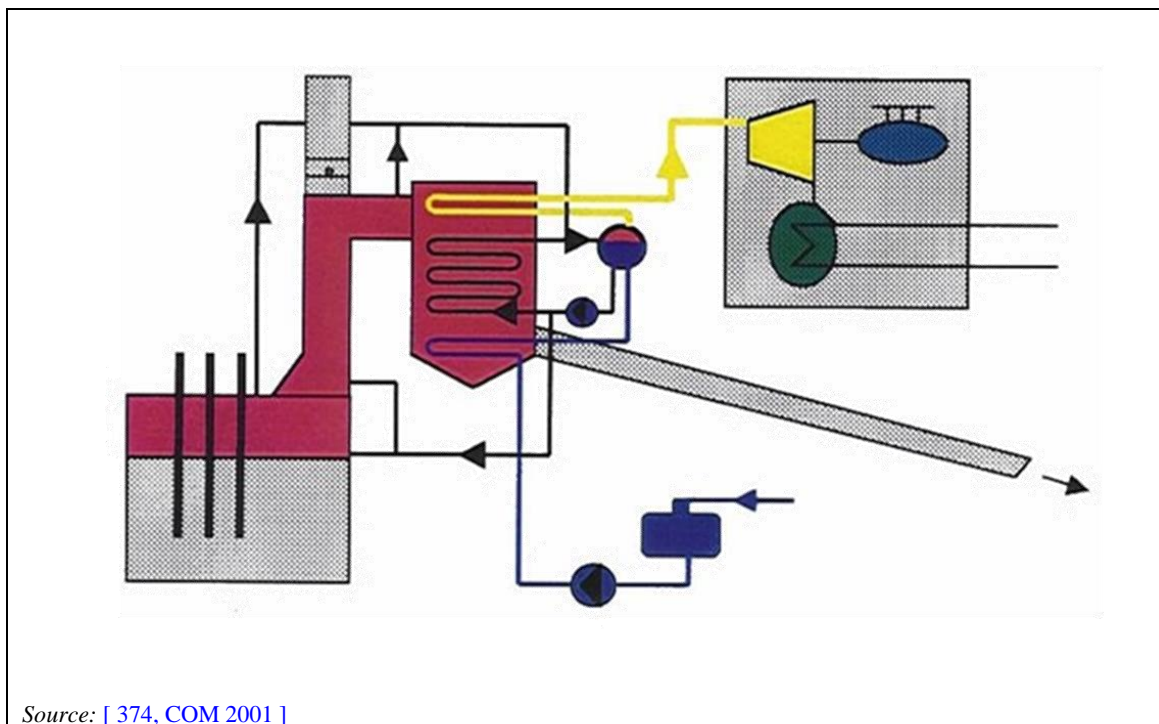
Figure 8.22: Energy recovery from a semi-closed furnace
