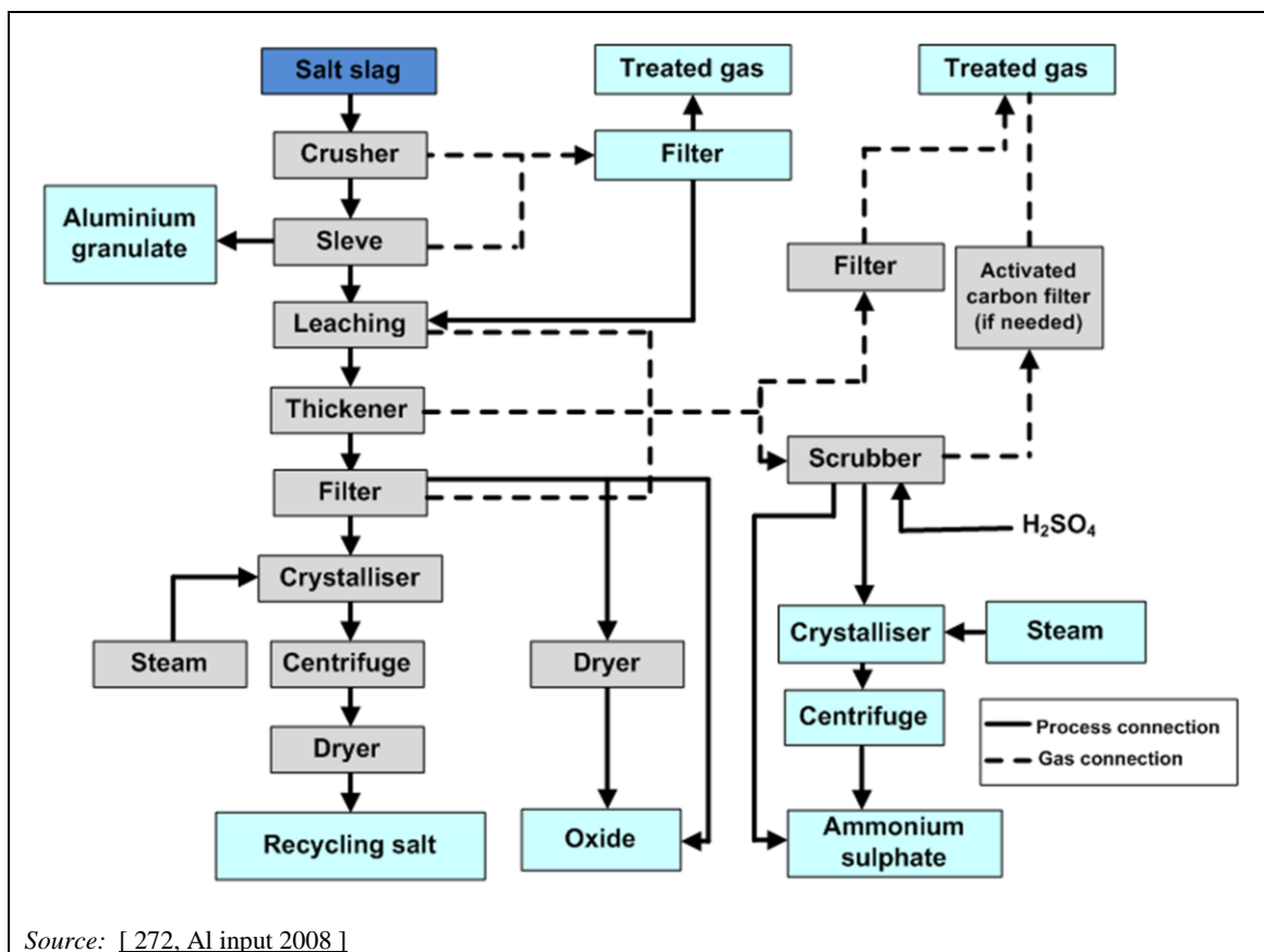
Figure 4.20: An example of the full salt slag recycling process
