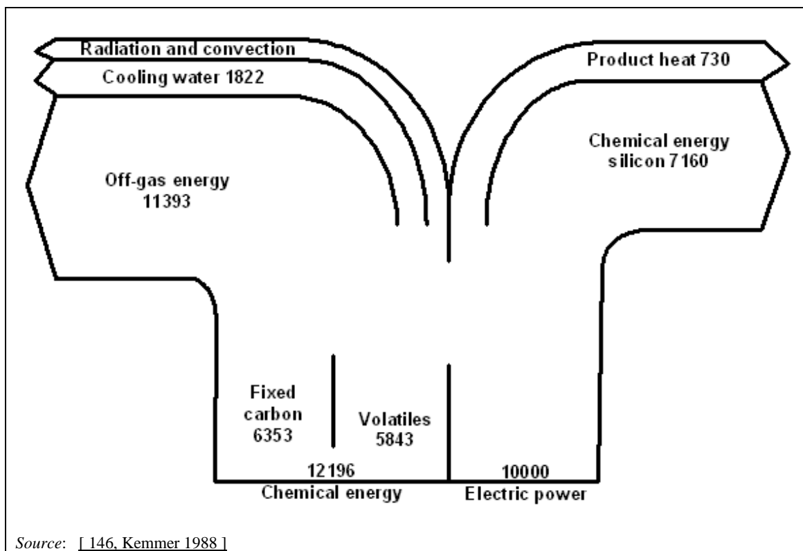
Figure 8.20: Energy flowsheet (in MW th ) in a 10 MW e silicon furnace
