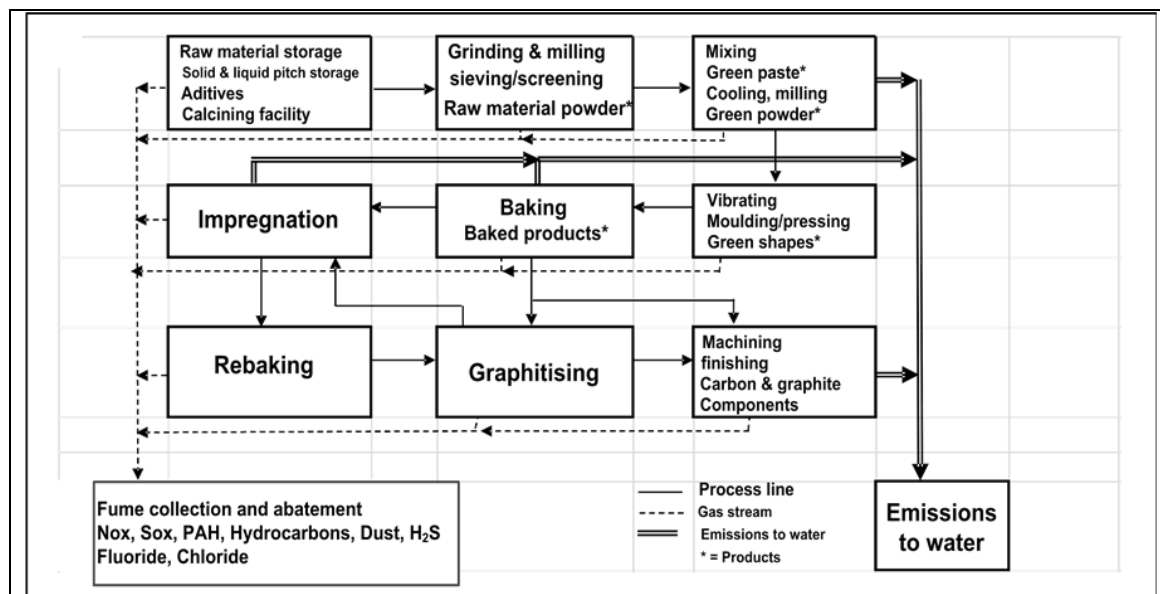
Figure 10.6: Generic emission diagram of the carbon and graphite production processes
