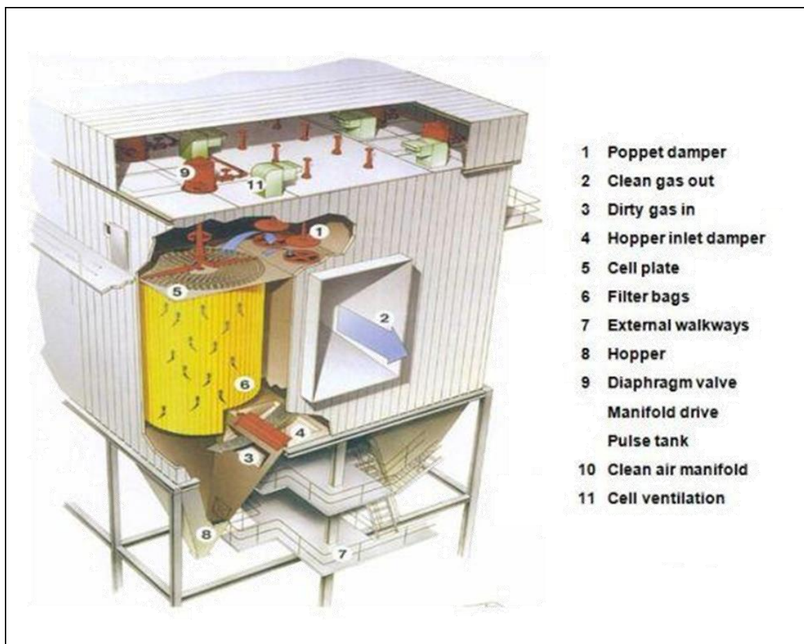
Figure 2.28: Low-pressure air pulsing cleaning system
