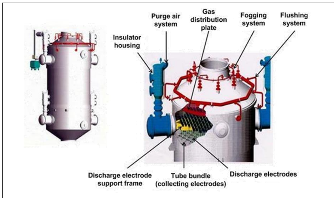
Figure 2.24: Wet electrostatic precipitator
