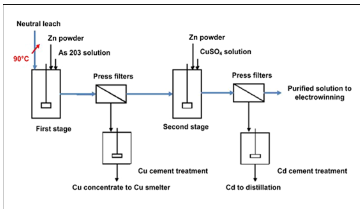
Figure 6.8: Example flowsheet for an As-based purification process for removal of Co and Ni
