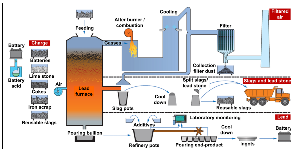
Figure 5.1: Outline of a typical shaft furnace lead-acid battery recovery process
