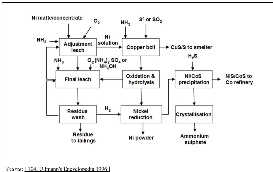
Figure 9.9: The Sherritt ammonia leach process
