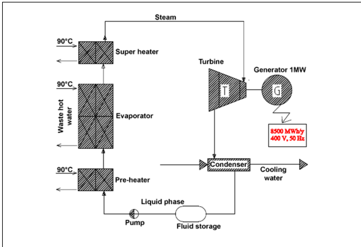
Figure 2.17: Electricity generation from low-grade heat
