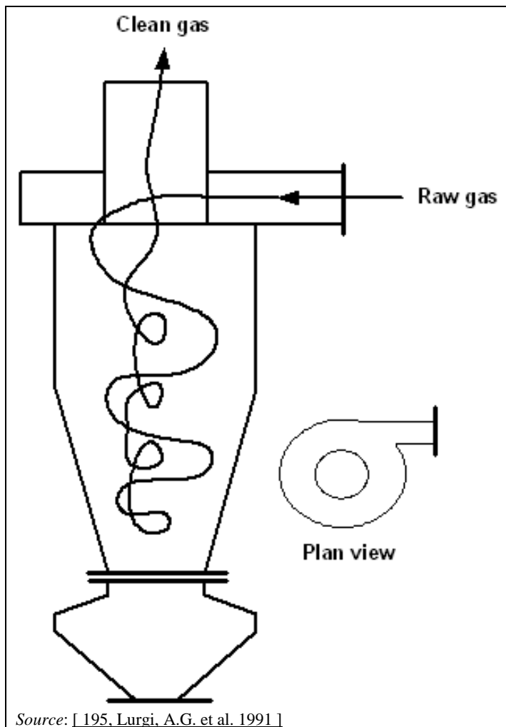
Figure 2.25: Arrangement of a cyclone
