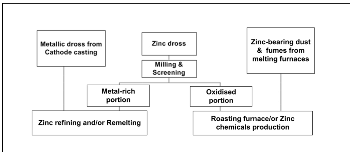
Figure 6.31: Flowsheet of a generic treatment for waste/residues produced during zinc melting
