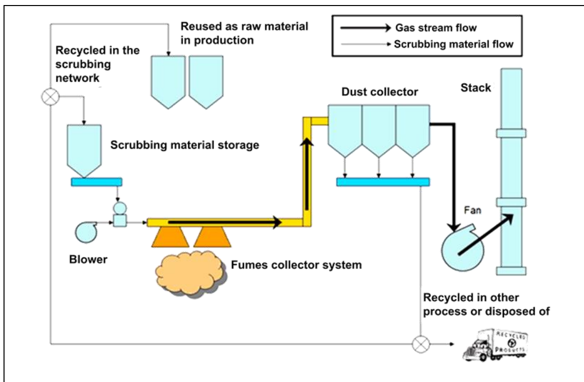
Figure 10.7: Dry adsorption scrubber with dust injection and dust removal
