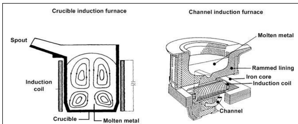
Figure 13.24: Induction furnaces
