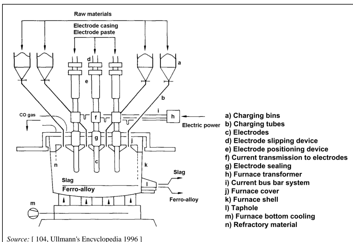
Figure 8.7: Closed electric arc ferro-manganese furnace operating with Søderberg electrodes
