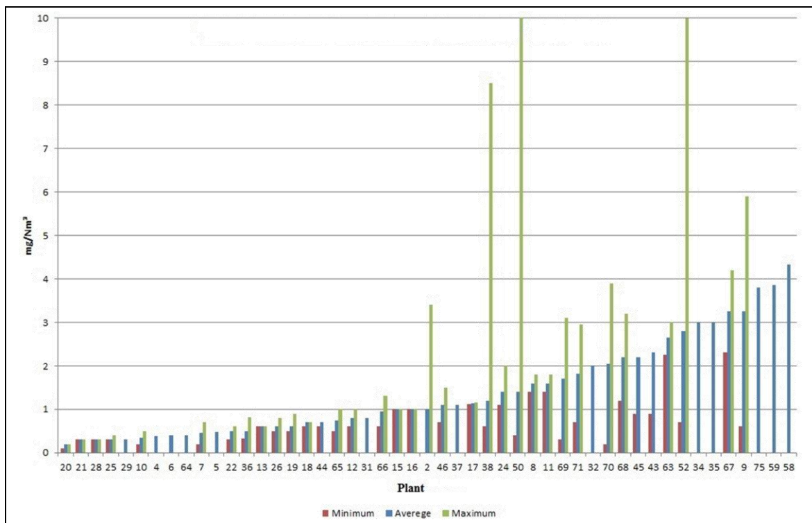
Figure 4.13: Dust emissions from the melting process in secondary aluminium production plants
