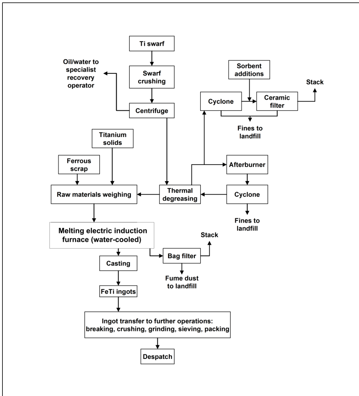
Figure 8.16: Flow diagram for ferro-titanium production
