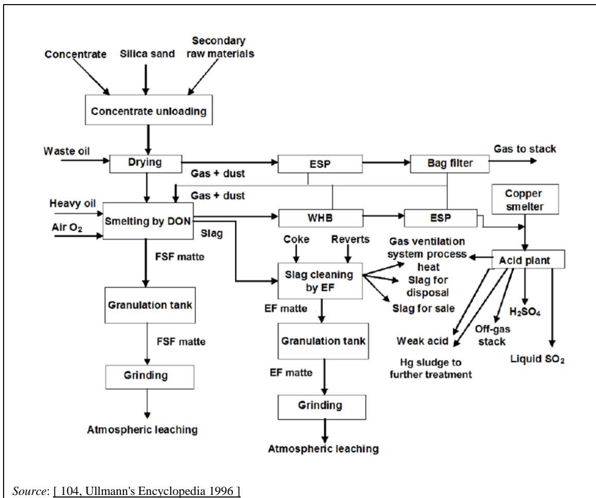
Figure 9.6: The Falconbridge process
