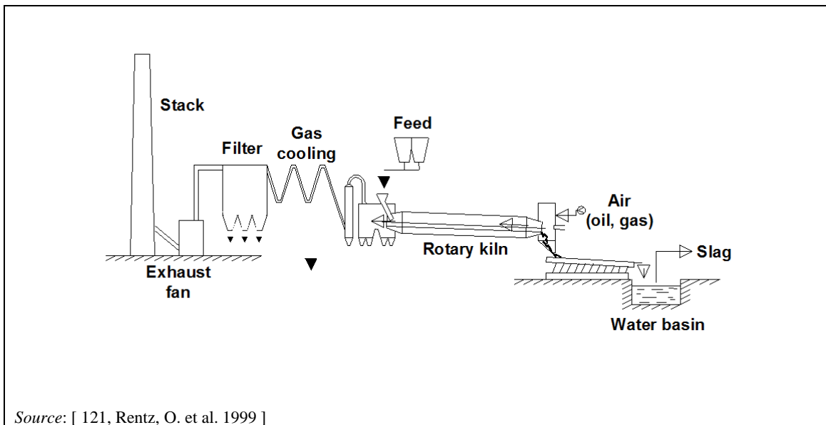
Figure 13.1: Rotary kiln
