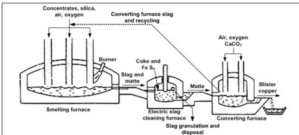
Figure 13.16: The Mitsubishi process
