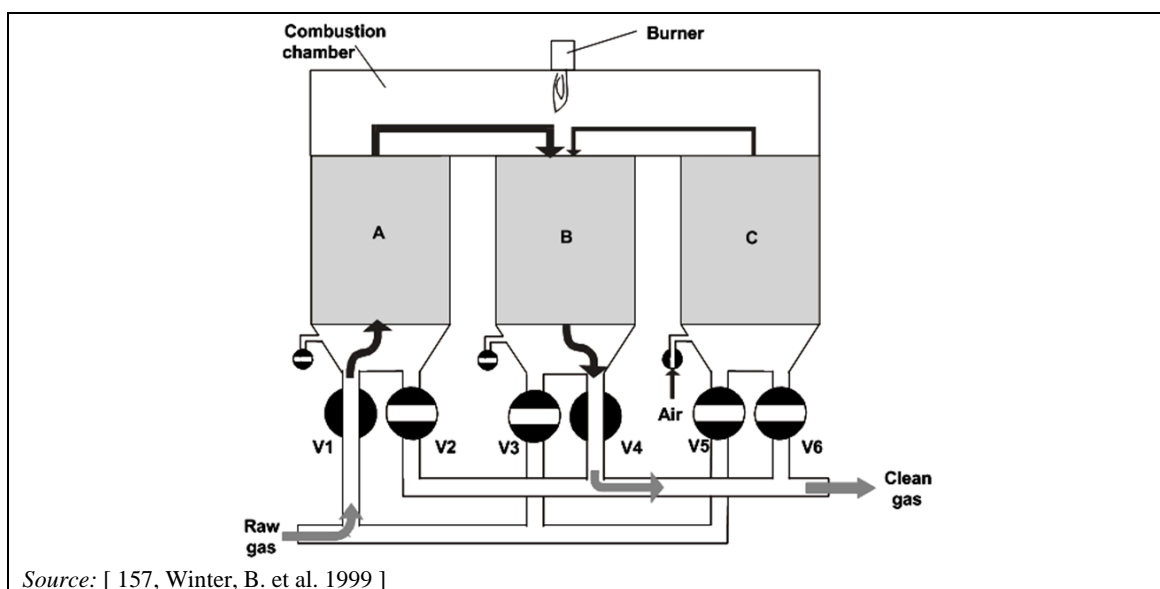
Figure 2.16: Regenerative afterburner
