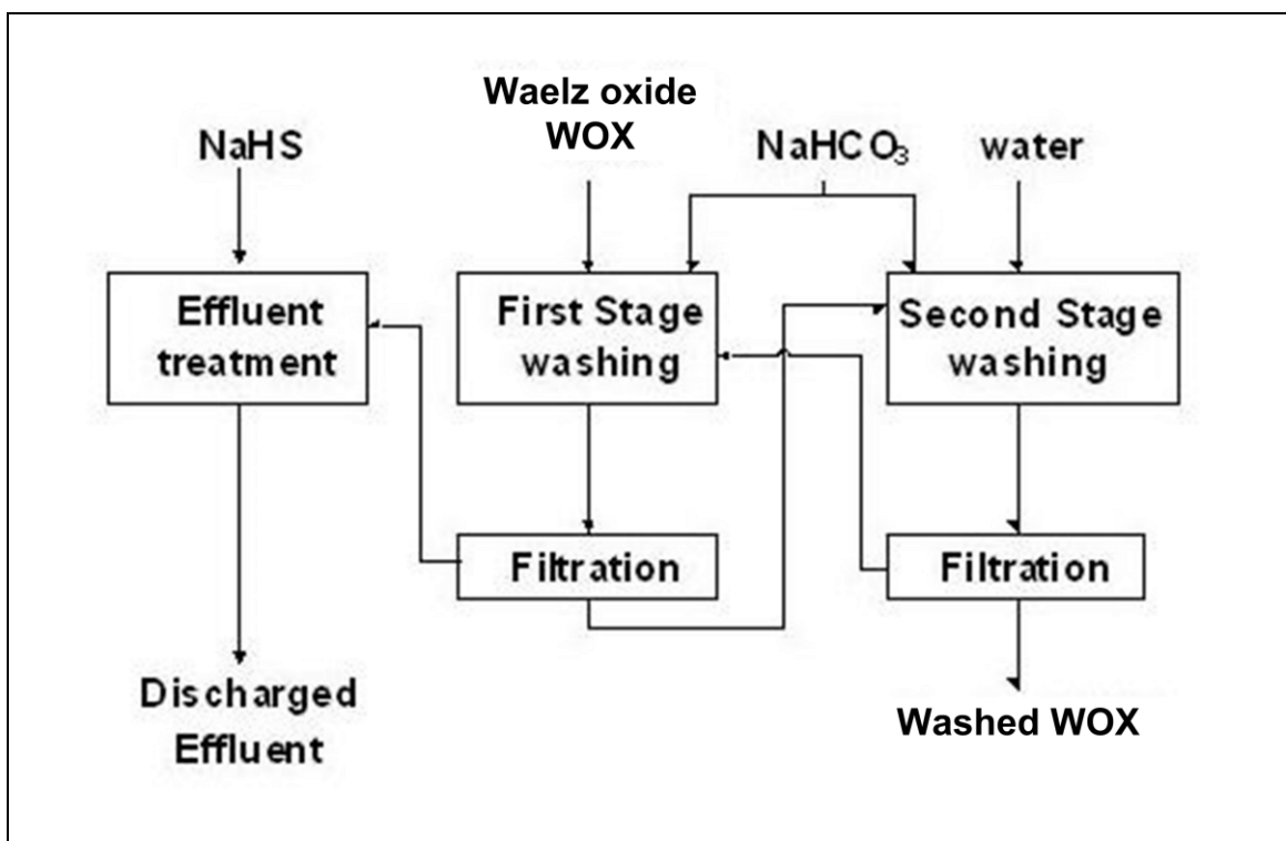
Figure 6.30: Diagram of a Waelz oxide two-stage countercurrent washing circuit
