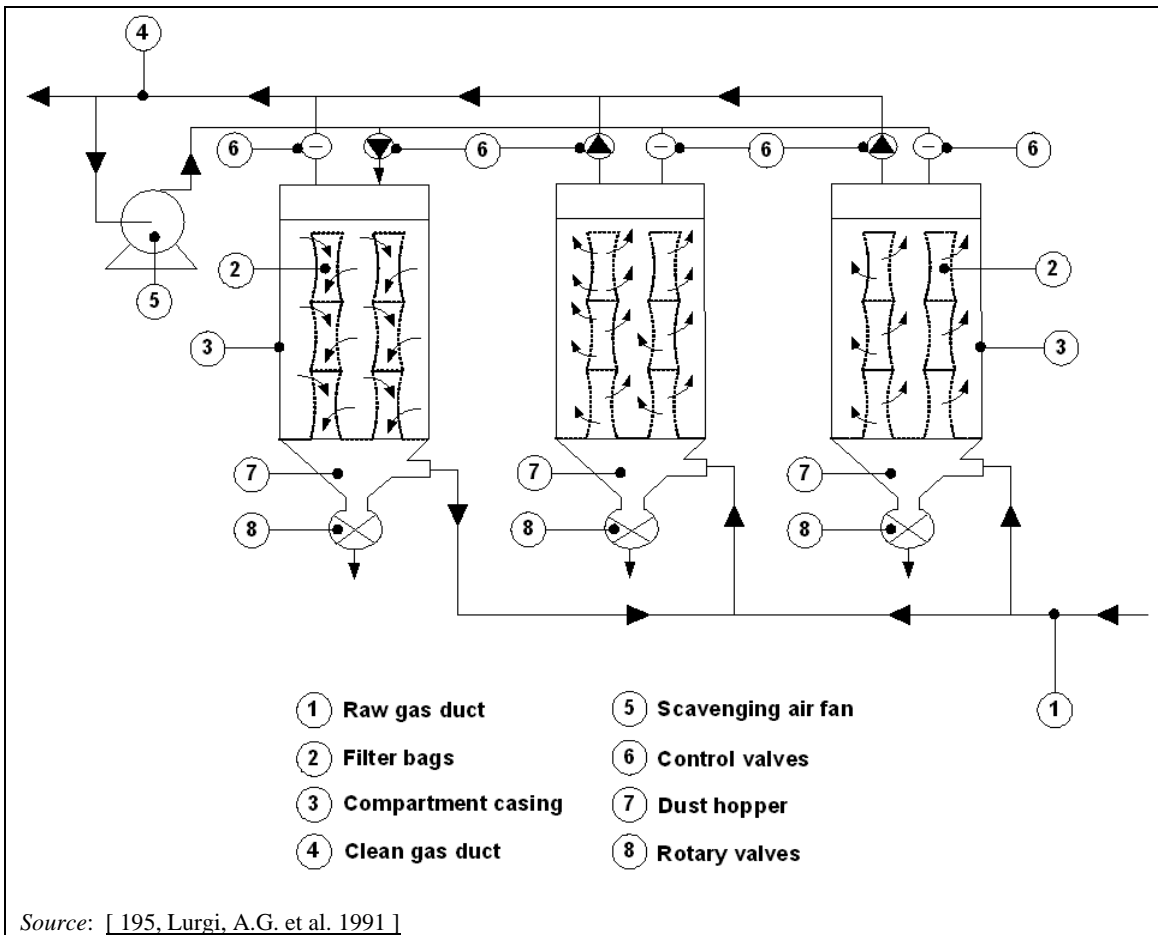
Figure 2.26: Reverse airflow bag filter (with one compartment in the cleaning cycle)
