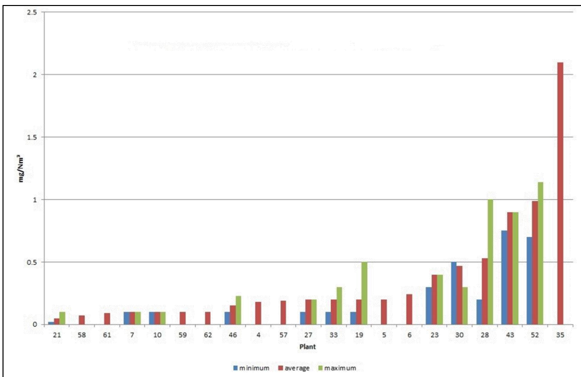
Figure 4.16: \text{Cl}_2 emissions in secondary aluminium production plants
