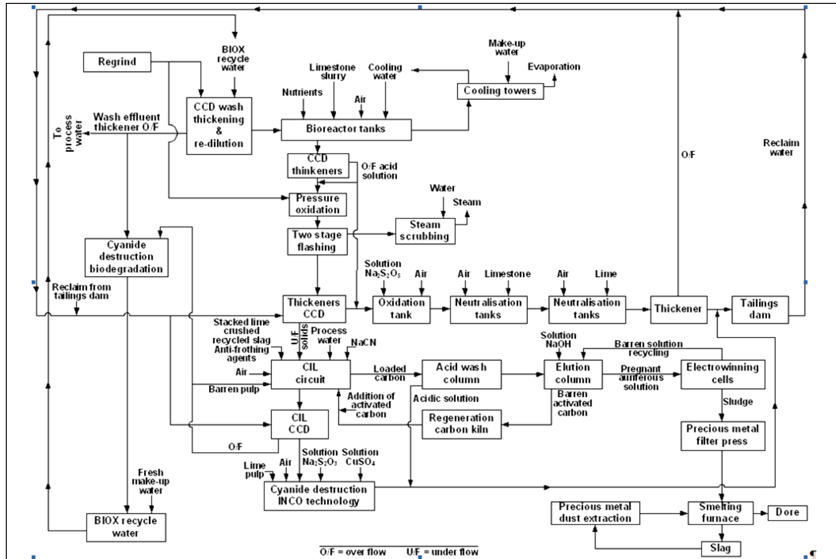
Figure 7.4: Metallurgical process flowsheet
