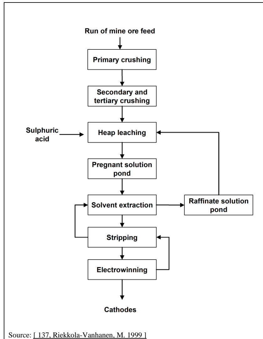
Figure 3.2: Flowsheet of a hydrometallurgical process
