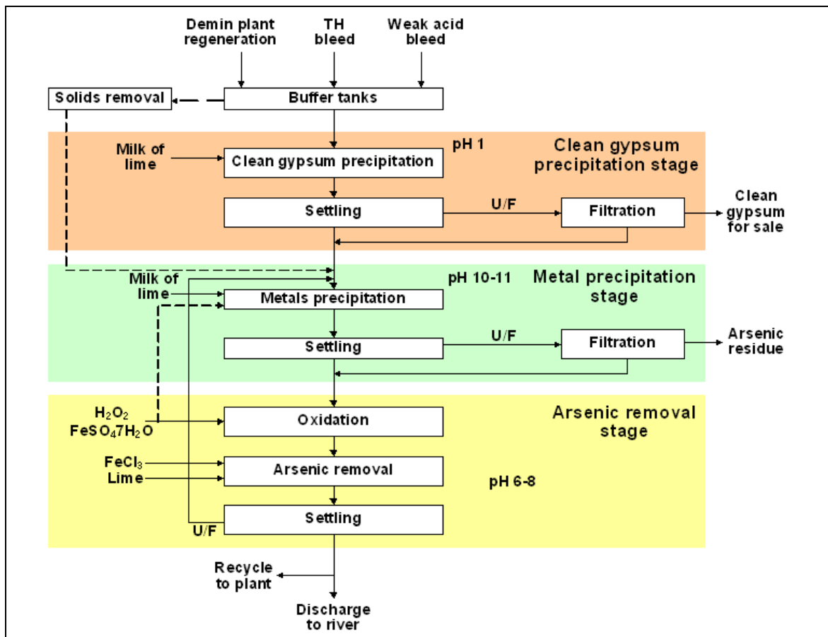
Figure 2.33: Treatment of weak acid
