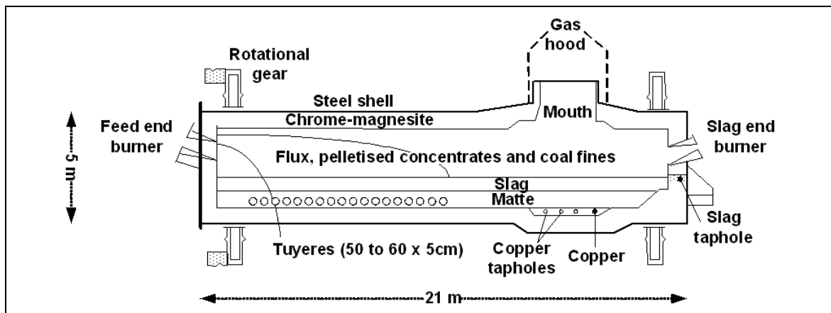
Figure 13.14: The Noranda reactor
